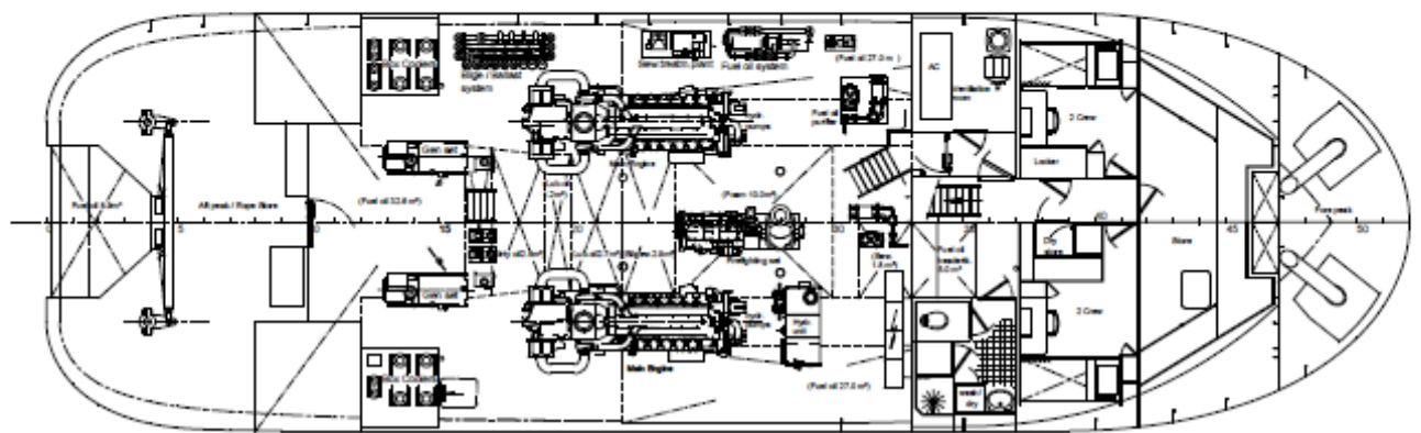
Below Maindeck
