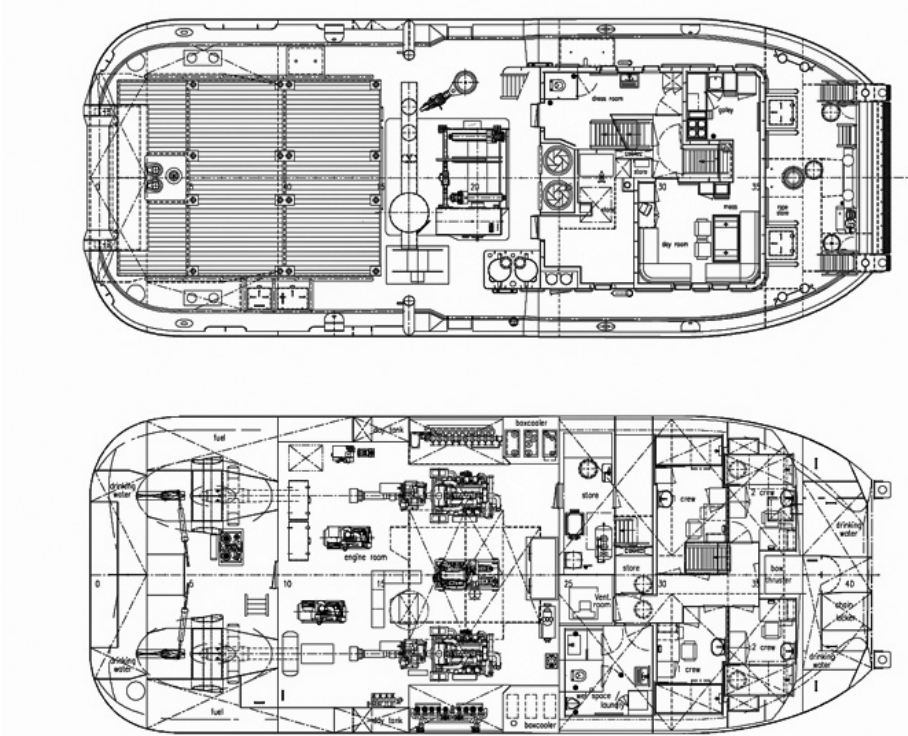
TOP VIEW DECK LEVEL
