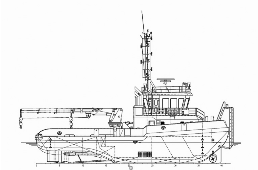
SIDE VIEW
