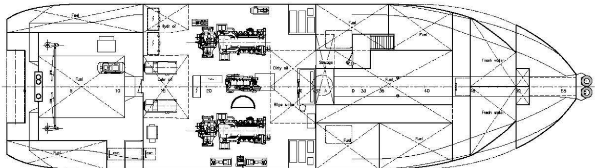
Below maindeck
